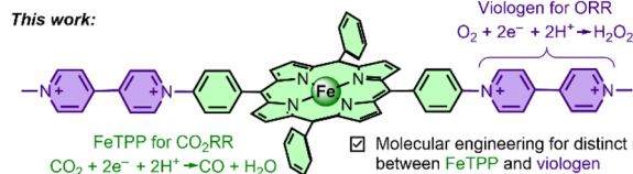
Scheme 1 Strategies for the electrocatalytic CO 2 RR in the presence of oxygen.
