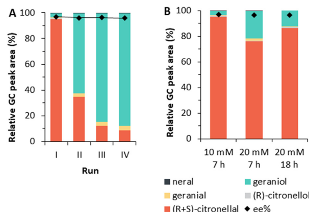
Fig. 5 Evaluation of (A) reusability of the immobilised enzymatic system and (B) increased substrate concentration, in the one-pot cascade. Reaction conditions: 50 mg dry resin immobilised CgrAlcOx and 50 mg dry resin co-immobilised OYE2 CFE and GDH CFE , 360 U mL -1 catalase, 3 μM HRP, 10 or 20 mM geraniol in acetone (final concentration, 1% v/v), 100 mM glucose, 1 mM NADP + , 100 mM KPi buffer pH 8.0 and 20% v/v heptane, 7 or 18 h, 25 °C, 180 rpm.
