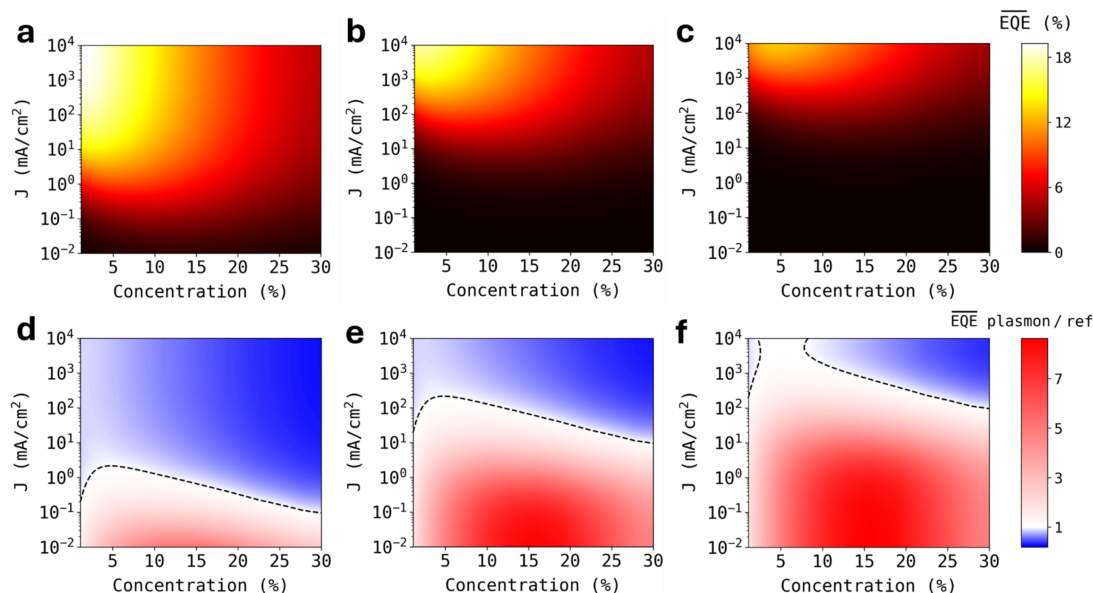
Fig. 5 (a–c) Calculated \overline{EQE} values for the plasmonic system as a function of the current density and NP concentration. Simulations are performed for three types of perovskite materials: high-performing ( k_1 = 10^6 \text{ s}^{-1} , k_2 = 10^{-9} \text{ cm}^3 \text{ s}^{-1} , k_3 = 10^{-28} \text{ cm}^6 \text{ s}^{-1} ), medium-performing ( k_1 = 10^7 \text{ s}^{-1} , k_2 = 10^{-9} \text{ cm}^3 \text{ s}^{-1} , k_3 = 10^{-28} \text{ cm}^6 \text{ s}^{-1} ) and low-performing ( k_1 = 10^7 \text{ s}^{-1} , k_2 = 10^{-10} \text{ cm}^3 \text{ s}^{-1} , k_3 = 10^{-28} \text{ cm}^6 \text{ s}^{-1} ). (d–f) Corresponding \overline{EQE} s enhancement maps compared to the reference (non-plasmonic) system. The dashed black line marks the unity contour, separating the region where \overline{EQE} is enhanced by plasmonic effects (lower red area) from the region where efficiency is reduced (upper blue area). At low current densities, these results highlight the potential for energy-efficient applications. The enhancement becomes more pronounced as nonradiative losses increase, illustrating the ability of plasmonic structures to induce defect tolerance and expand the operational versatility of PeLEDs.
