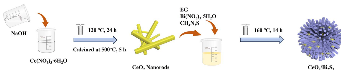
Scheme 1 Schematic illustration of the synthesis of CeO 2 /Bi 2 S 3 photocatalysts.
