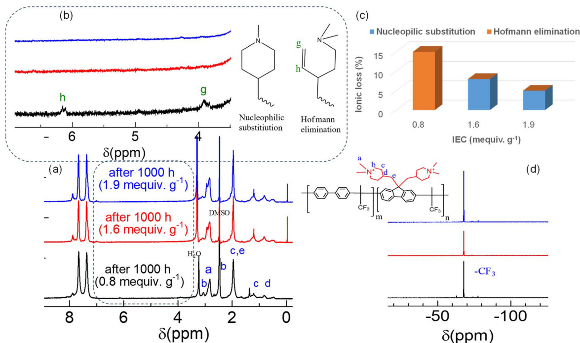
Fig. 8 (a) Post-test 1 H NMR spectra of QBPh-Pip membranes after 1000 h in 8 M KOH at 80 °C, (b) magnified 1 H NMR spectra, (c) IEC loss (%) estimated from the NMR integrals as a function of IEC, and (d) 19 F NMR spectra of the post-test QBPh-Pip.
