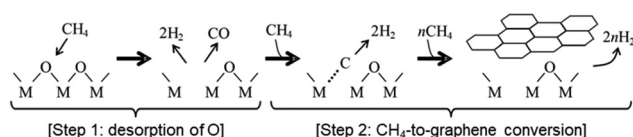
Fig. 3 Mechanism of graphene formation via CVD using CH 4 as a precursor on \gamma -Al 2 O 3 and MgO (M = Al or Mg).
