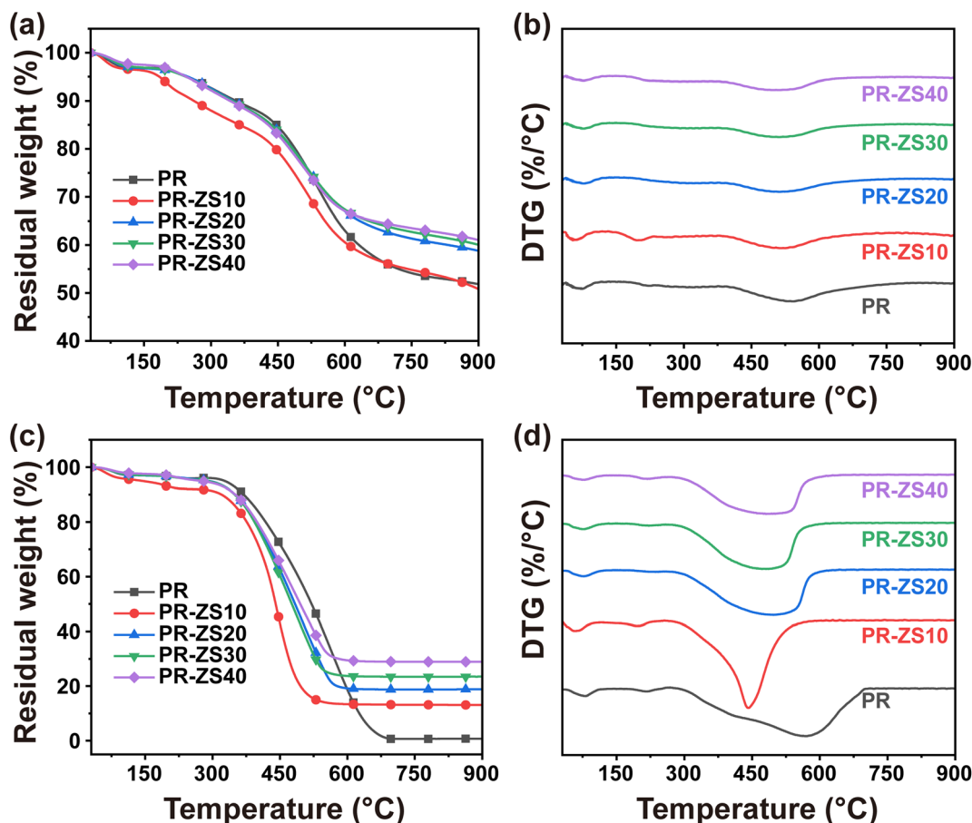
Fig. 4 TGA and DTG curves of PR and PR-ZS aerogels in (a and b) N 2 and (c and d) air atmospheres.
