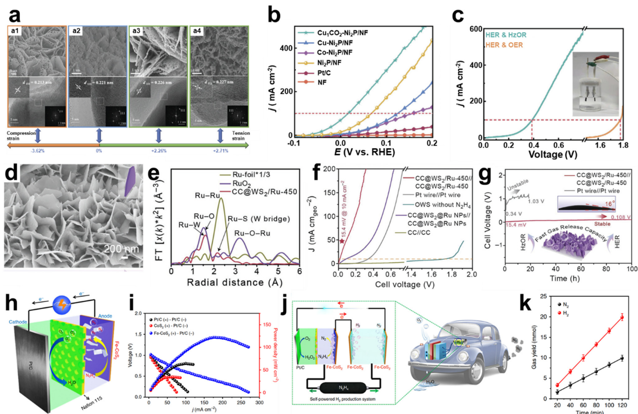
Fig. 11 Hydrazine oxidation reaction (HzOR). (a) SEM (top) and HRTEM (bottom) images of catalysts. a1: Cu 1 Co 2 -Ni 2 P/NF, a2: Ni 2 P/NF, a3: Co-Ni 2 P/NF, and a4: Cu-Ni 2 P/NF. (b) Polarization curves of various catalysts in 1 M KOH with 0.1 M N 2 H 4 . (c) Polarization curves of Cu 1 Co 2 -Ni 2 P/NF as both an anode and a cathode in 1 M KOH with or without 0.1 M N 2 H 4 . (d) SEM image of CC@WS 2 /Ru-450. (e) FT-EXAFS spectra of CC@WS 2 /Ru-450, RuO 2 , and Ru-foil. (f) Polarization curves of CC@WS 2 /Ru-450 as both an anode and a cathode in 1 M KOH with or without 0.5 M N 2 H 4 . (g) Stability test of HzOR-assisted water electrolysis using CC@WS 2 /Ru-450||CC@WS 2 /Ru-450 and Pt wire||Pt wire (inset: contact angle test). (d–g) Reprinted with permission. 128 Copyright 2023, Wiley-VCH GmbH. (h) Schematic illustration of DHZFCs using Fe-CoS 2 nanosheets as the anode and commercial 40 wt% Pt/C as the cathode with O 2 as the oxidizing reagent. (i) Current density–voltage profiles and current density–power density profiles for the DHZFC. (j) Schematic illustration of a self-powered H 2 production system integrated with DHZFC and OHZS systems. (k) N 2 and H 2 generation in the system with 5.3 M hydrazine. (h–k) Reprinted with permission. 130 Copyright 2018, Springer Nature.
