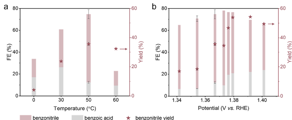
Fig. 7 PhCN electrosynthesis over a range of temperatures. FE values and PhCN yields of the electro-oxidative coupling of BnOH and \text{NH}_3 on Ni foam for 3 h under different (a) temperatures (20 mM BnOH, 1 M \text{NH}_3 , pH 13, the applied potentials were chosen based on LSV curves in ESI Fig. S29†) and (b) potentials (20 mM BnOH, 1 M \text{NH}_3 , pH 13, 50 °C). The error bars denote the standard deviation of data from two independent experiments.
