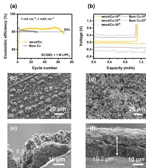
Fig. 3 Electrochemical performances of Li|Cu half cells at 1.0 mA cm -2 and 1.0 mA h cm -2 : (a) coulombic efficiency values during cycling and (b) charging-discharging curves at different cycles. Morphologies of deposited Li after 5 cycles in Li|Cu half cells with (c and e) or without (d and f) the wood host.
