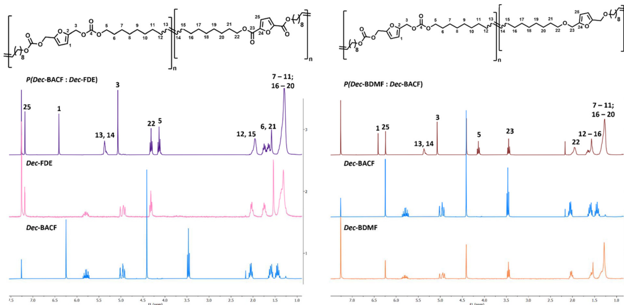
Fig. 9 Co-polymer NMR analysis ( \text{CDCl}_3 ) for \text{P(Dec-BACF : Dec-FDE)} and \text{P(Dec-BDMF : Dec-BACF)} .
