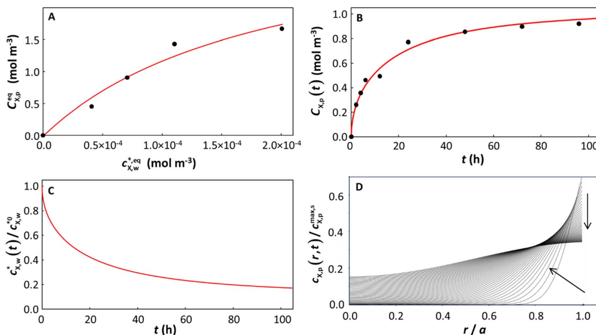
Fig. 3 Equilibrium and kinetic features of a system with considerable depletion of X in the bulk solution: sorption of naphthalene on polyethylene terephthalate particles ( a = 1.5 \times 10^{-3} m). The panels correspond to (A) equilibrium sorption isotherm; (B) kinetic sorption curves; (C) solution depletion profile; and (D) temporal evolution of the normalized intraparticle concentration profiles, with the direction of increasing time indicated by the arrow. In (D), the timescale between two plotted concentration profiles is \Delta t = 16\,021 s, starting at t = 16\,021 s. The condition at t = 0 (not shown) corresponds to plastic particles free of contaminants and to the initial bulk medium condition c_{X,w}^*(t=0) = c_{X,w}^{*,0} . The Langmuir isotherm best described the equilibrium data, and \tau was the only parameter optimized to fit the sorption curves (see Table S1† for the pertaining parameters). The isotherm curve (A) shows the experimental data (black circles) 59 and the best fit obtained according to the Langmuir sorption isotherm (eqn (1)–(2b), red curve, adjusted parameters: K_{p,w}^H and c_{X,p}^{\max,s} ); the kinetic sorption curve (B) shows the experimental data (black circles) 59 and numerically computed values, eqn (1)–(2b), (3)–(5), (7) and (8) (red curve); and the depletion profile (C) shows the values obtained from numerical computation, eqn (1)–(2b), (3)–(5), (7) (red curve). The maximal extent of bulk depletion is 87% in the kinetic sorption data, and from the fitted \tau of 2225.2 h, the derived diffusion coefficient is D_{X,p} = 2.81 \times 10^{-13} \text{ m}^2 \text{ s}^{-1} .
