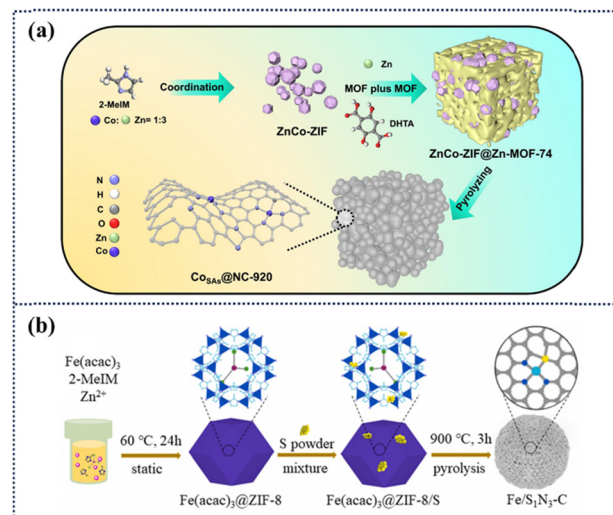
Fig. 13 Synthesis methods for single-atom catalysts: CoSAs@NC-920 and Fe-SN-C. (a) Illustration of the synthetic procedure of CoSAs@NC-920. 81 Copyright 2024 Elsevier. (b) Scheme of the synthesis of Fe-SN-C. 87 Copyright 2024 Elsevier.
