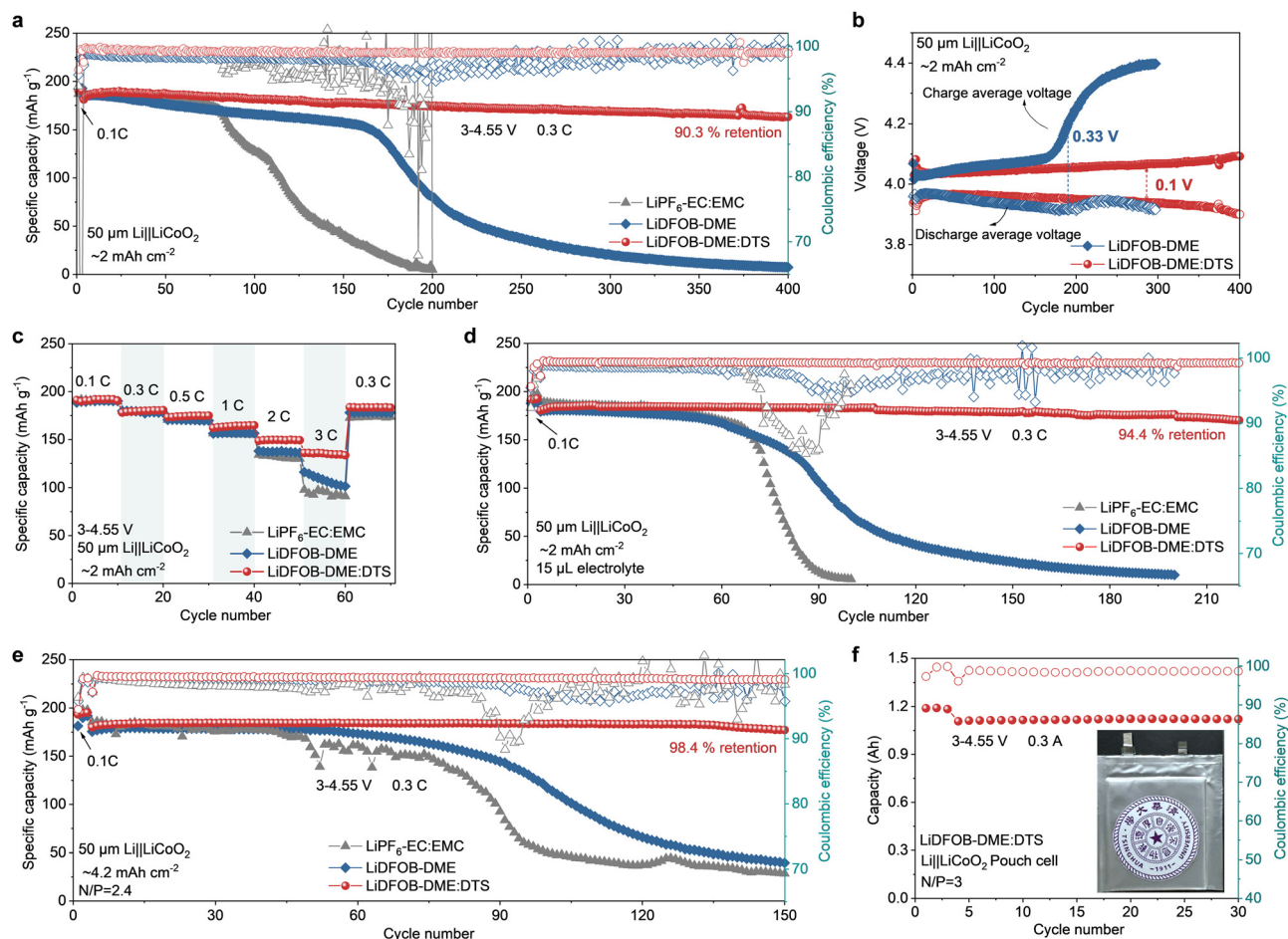
Fig. 3 Electrochemical performance of \text{Li}||\text{LiCoO}_2 cells. (a) Cycling performance of \text{Li}||\text{LiCoO}_2 cells with different electrolytes in the voltage range of 3–4.55 V at 25^\circ\text{C} . (b) The charge and discharge average voltage of \text{Li}||\text{LiCoO}_2 batteries with different electrolytes during cycling. (c) Rate performance of \text{Li}||\text{LiCoO}_2 cells under different C rates. (d) Cycling performance of \text{Li}||\text{LiCoO}_2 cells with the 15 \mu\text{L} electrolyte. (e) Cycling performance of \text{Li}||\text{LiCoO}_2 cells with an N/P ratio of 2.4 in the LiDFOB–DME:DTS electrolyte. (f) Cycling performance of \text{Li}||\text{LiCoO}_2 pouch cells with the LiDFOB–DME:DTS electrolyte. The inset shows the optical image of the pouch cell.
