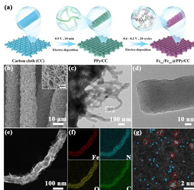
Fig. 1 (a) Schematic illustration for the synthesis of \text{Fe}_{\text{SA}}/\text{Fe}_{\text{AC}}@\text{PPy}/\text{CC} . (b) SEM, (c) TEM, (d) HRTEM, (e) and (f) elemental mapping and (g) HAADF-STEM images of iron clusters (red circles) coupled with iron single atoms (blue circles) of \text{Fe}_{\text{SA}}/\text{Fe}_{\text{AC}}@\text{PPy}/\text{CC} .
