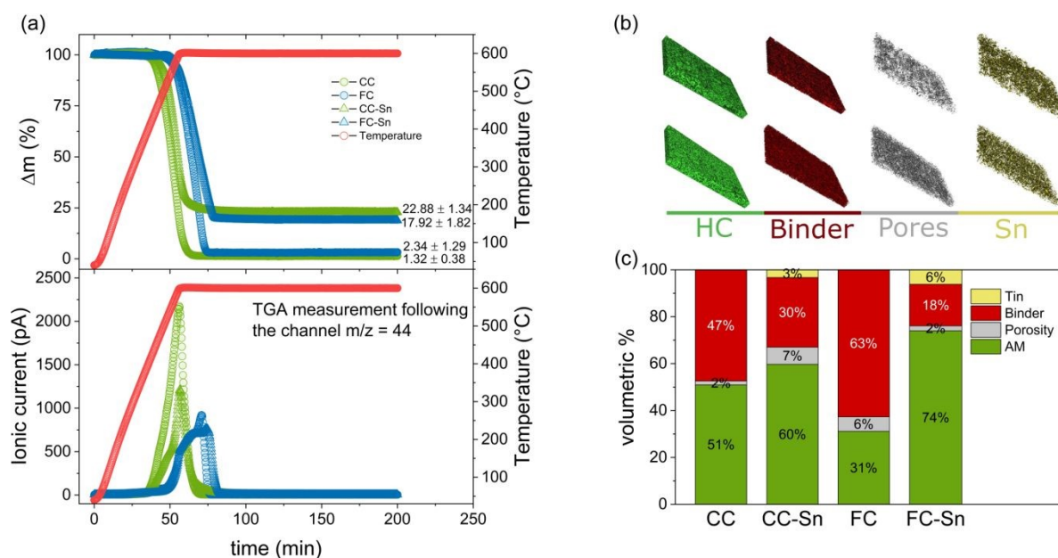
Figure 3: (a) Residual mass in the HCs and composites after TGA-MS in air and relative ionic current given by \text{CO}_2 evolution. (b) 3D XRM reconstructions of the section of composite electrodes (CC-Sn on top and FC-Sn on the bottom). (c) Volumetric % of electrodes components.
