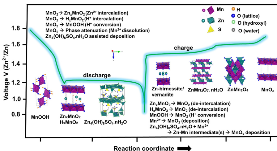
Fig. 2 Despite showing many similarities in their electrochemical charge-discharge curves, different polymorphs of MnO 2 with or without Mn 2+ additives in the ZnSO 4 electrolyte have been proposed to have diverse mechanisms in the literature. These mechanisms with the respective intermediate/end products have been analyzed through plausible operando and non-operando techniques.
