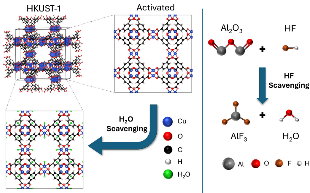
Fig. 2 Scavenging mechanism for H 2 O and HF by HKUST-1 and Al 2 O 3 nanoparticles, respectively.
