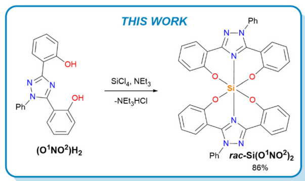
Scheme 1 Structures of Deferasirox (top, left), the previously studied NHC pincer-type \text{O}^{\wedge}\text{C}^{\wedge}\text{O} proligand (\text{OCO})\text{H}_3 (top, right) and the synthetic strategy for obtaining the \text{Si}(\text{iv}) complex of the current work (bottom).
