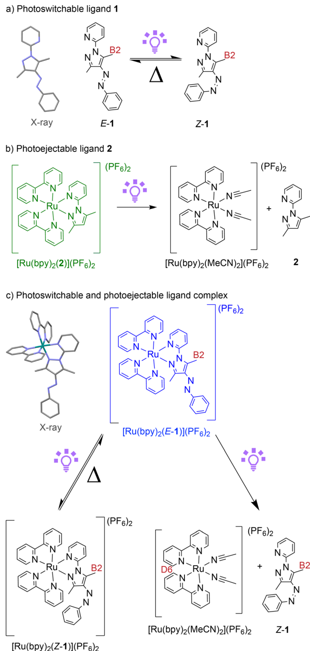
Fig. 1 (a) Photoswitchable ligand, 1, and its UV light triggered photo-switching. (b) Ruthenium complex, [\text{Ru}(\text{bpy})_2(2)](\text{PF}_6)_2 , containing non photoswitchable ligand 2 and its photoejection triggered by UV light. (c) Ruthenium complex, [\text{Ru}(\text{bpy})_2(\text{E-1})](\text{PF}_6)_2 , containing photo switchable ligand 1 and its photoejection and photo isomerisation triggered by UV light. Chosen hydrogen environments are labelled in red.
