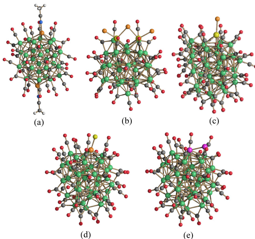
Fig. 7 Ni-carbide MCCs decorated by Cu and Cd-based fragments: (a) [H_2Ni_{30}C_4(CO)_{34}\{Cu(MeCN)\}_2]^{4-} (green, Ni; orange, Cu; grey, C; red, O; blue, N; white, H); (b) [Ni_{36}C_8(CO)_{36}(Cd_2Cl_3)]^{5-} , (c) [Ni_{42+x}C_8(CO)_{44+x}(CdCl)]^{7-} ( x = 0.19 ) (green, Ni; yellow, Cd; orange, Cl; grey, C; red, O); (d) [HNi_{42}C_8(CO)_{44}(CuCl)]^{7-} and (e) [HNi_{43+x}C_8(CO)_{45+x}]^{7-} (two CO ligands with partial occupancy factors have not been located) (green, Ni; purple, Ni with partial occupancy factor; orange Cu; yellow, Cl; grey, C; red, O). Hydride ligands have not been located by SC-XRD. Adapted from ref. 84 and 85 with permission from Springer and Elsevier.
