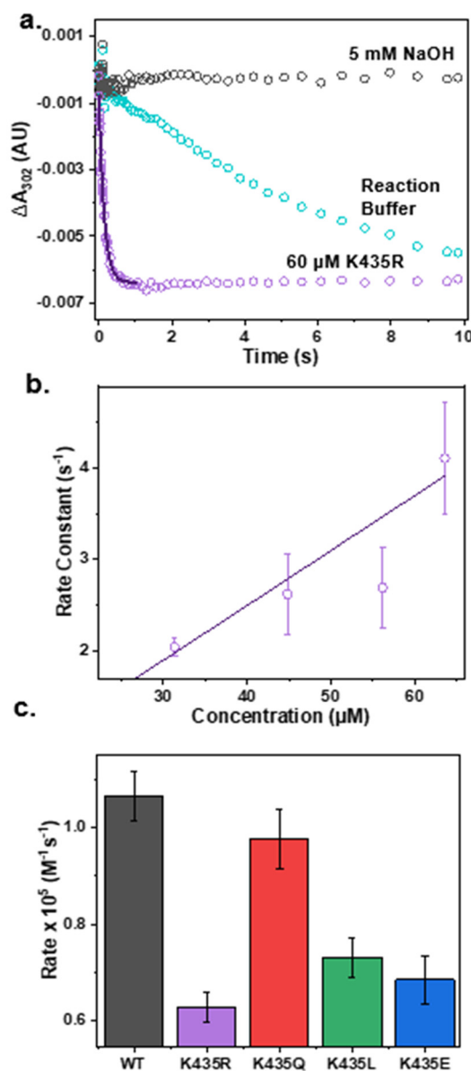
Fig. 3 Removal of \text{ONOO}^- by Cu(I)-E2 mutants. (a) The reduction of peroxynitrite was monitored by the decrease in absorption at 302 nm using stopped-flow spectroscopy in 5 mM NaOH (gray), reaction buffer (blue), and in the presence of the Cu(I)-E2 K435R mutant in the reaction buffer (purple) with its respective linear fit (black). (b) Pseudo-first-order rate constants for peroxynitrite reduction as a function of K435R concentration. (c) Second order reaction rates for \text{ONOO}^- removal by Cu(I)-E2 and mutants.
