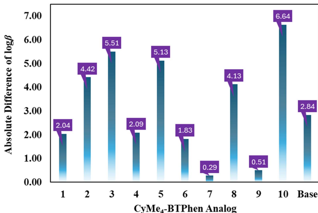
Fig. 7 Transfer learning results using the model trained on 803 BTBP ligands for predicting log \beta values of 10 + 1 CyMe 4 -BTPhen analogs (their structures are shown in ESI Section S5 and Fig. S10†). The y-axis shows the absolute difference between the DFT-computed and the predicted log \beta values.
