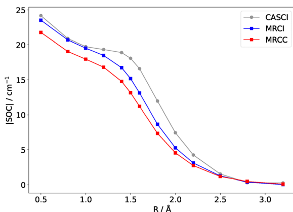
Fig. 1 Run of the computed spin–orbit coupling matrix elements between the X 3 Σ − and the c 1 Π state of NH. The computations use the cc-pCVDZ basis set, all electrons were correlated. For MRCC, the averaged value is plotted, see text.
