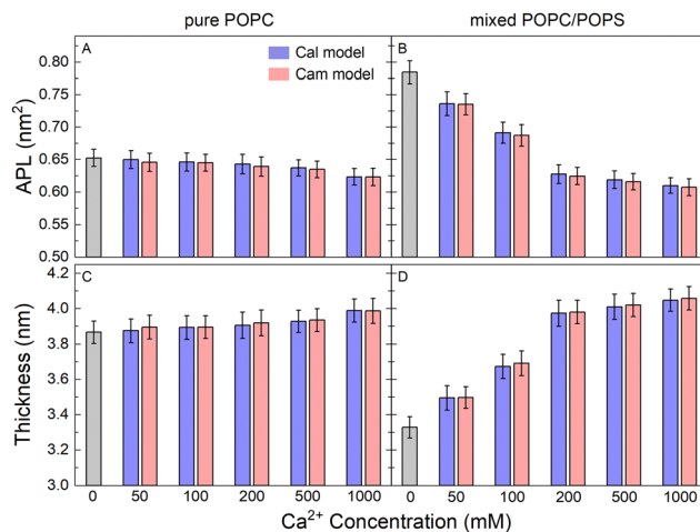
Fig. 2 Structural properties of the simulated lipid bilayers. Area per lipid (APL) for pure POPC (A) and mixed POPC/POPS (B) lipid bilayers with increasing \text{CaCl}_2 concentrations. The APL and bilayer thickness were calculated by the SuAVE software 39,40 (C) and (D).
