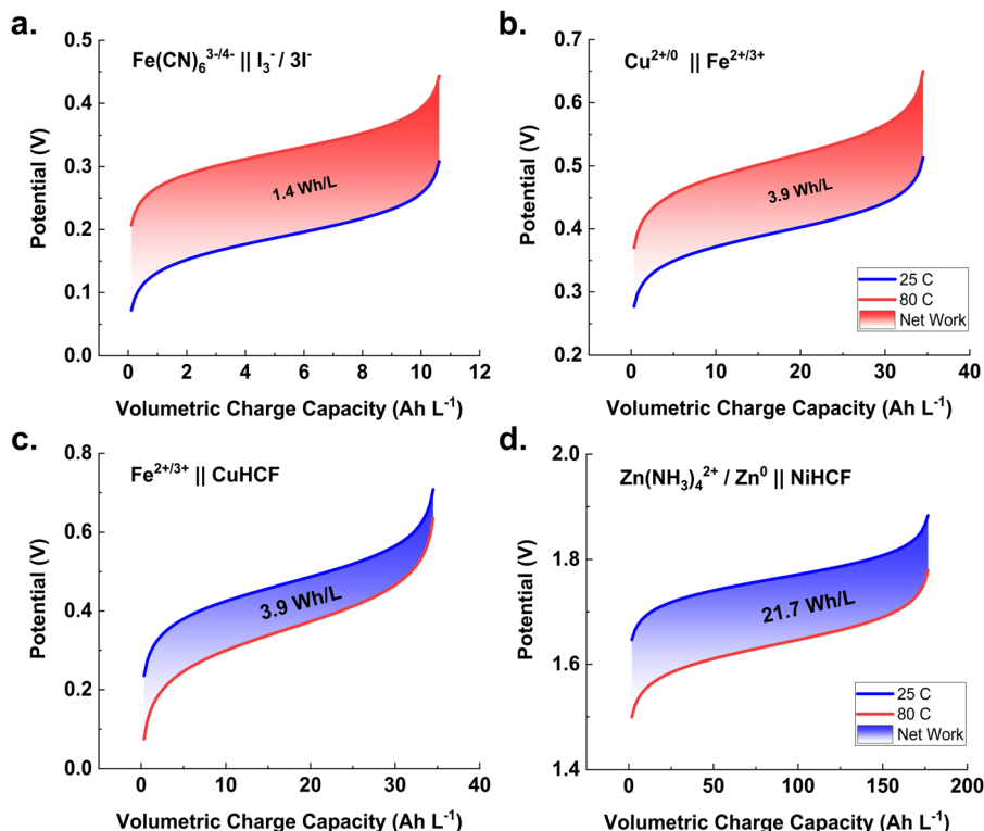
Fig. 4 Cell voltage vs. charge capacity plot of the TREC cycle between 25 °C and 80 °C for the screened redox couple combinations – (a) \text{Fe(CN)}_6^{3-/4-} \parallel \text{I}_3^- / 3\text{I}^- , (b) \text{Cu}^{2+/0} \parallel \text{Fe}^{2+/3+} , (c) \text{Fe}^{2+/3+} \parallel \text{CuHCF} , and (d) [\text{Zn(NH}_3)_4]^{2+} / \text{Zn}^0 \parallel \text{NiHCF} . Both thermodynamic cycles shift the charging curves higher (a) and (b) or lower (c) and (d) than the discharging curves; therefore, net work is produced during these cycles because of the voltage differences. The charge curves are theoretical and exclude some aspects only measurable in a practical system, such as ohmic losses.
