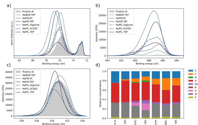
Fig. 4 XPS deconvolution results of the spectra shown in Fig. S6–S8 (ESI†). The spectra shown here are energy calibrated to the “bulk”-signal of aluminium Al2p positioned to 72.7 eV, (a) Al2p, (b) F1s, and (c) O1s core levels. The relative atomic concentrations are shown in (d), this estimation is based on the models in Fig. S6–S8 (ESI†). The spectra in (a) have been area normalized to the intensity that was believed to be caused by the pure aluminium (“bulk” aluminium).
