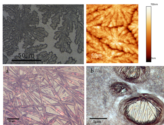
Fig. 6 Top left: Optical microscopy image of a glassy slide modified with ds-DNA (50 × objective lens) and top right: AFM topography for a 4 mM solution of ds-DNA drop casted on a Si substrate. Bottom left: Na[o-FESAN] dry solution (20 × objective lens) and bottom right: CT-dsDNA/Na[o-FESAN] nanohybrid (100 × objective lens).
