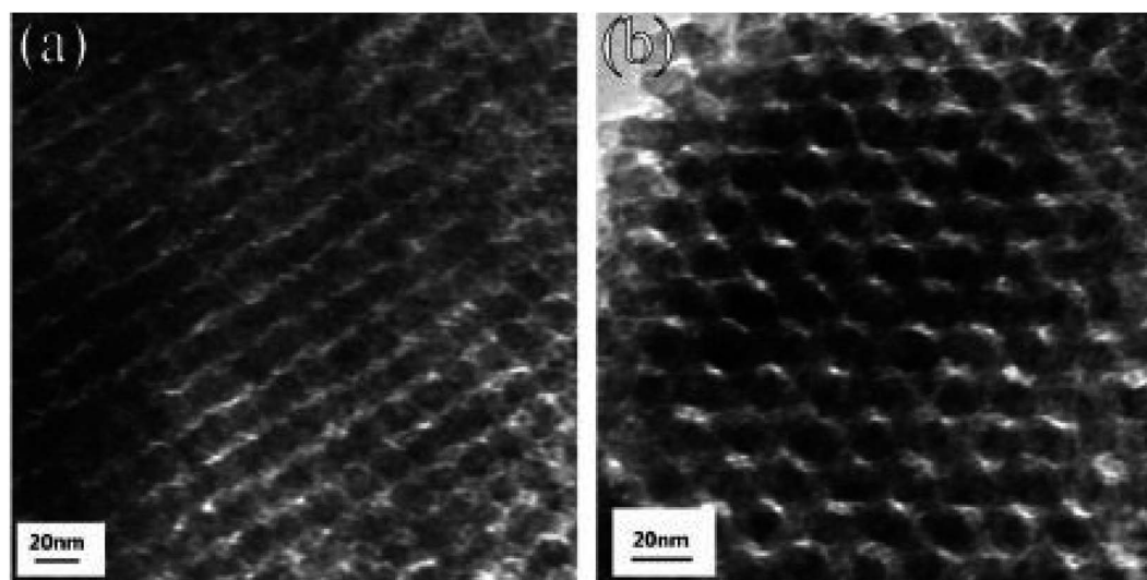
Fig. 8 HRTEM images of (a) 50^\circ \text{C-In}_2\text{O}_3 and (b) 100^\circ \text{C-In}_2\text{O}_3 . Copyright 2019, Elsevier. 56
