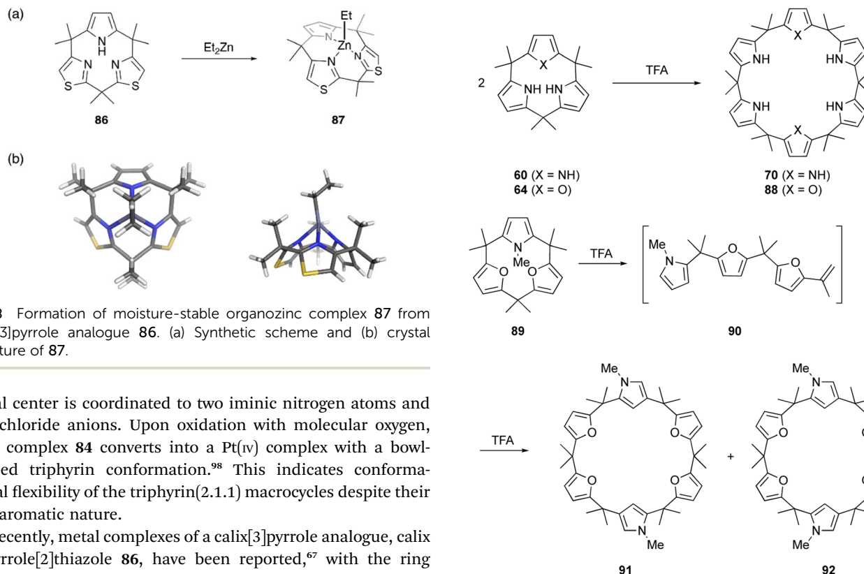
Scheme 14 Strain-induced ring expansion of calix[3]pyrrole analogues.
