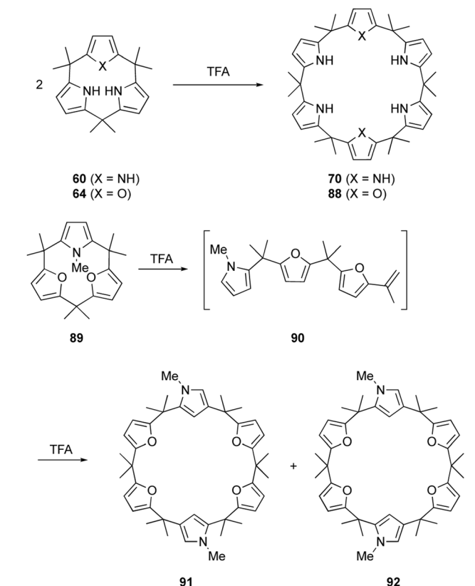
Scheme 14 Strain-induced ring expansion of calix[3]pyrrole analogues.
