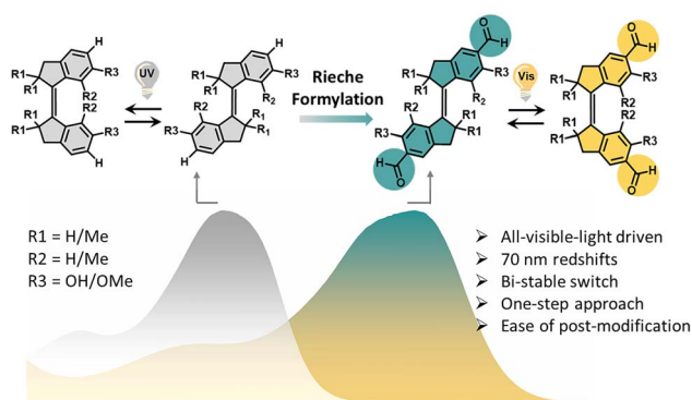
Fig. 1 Molecular structures of the stiff-stilbenes S1–S6 controlled using UV light and visible light, respectively, and cartoon representation of the absorption band of stiff-stilbenes substituted with aldehydes ( S2 , S4 , and S6 ) and those without formyl group ( S1 , S3 , and S5 ).
