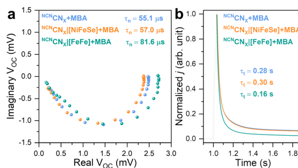
Fig. 5 (a) Nyquist plots of IMVS response. (b) Normalized TPC response with corresponding exponential fitting curves. Conditions: 20 mL anaerobic MOPS buffer (0.1 M, pH 7) containing 50 mM 4-MBA, Ag/AgCl (3 M NaCl) reference electrode, Pt mesh counter electrode, AM 1.5G irradiation, 25 °C.
