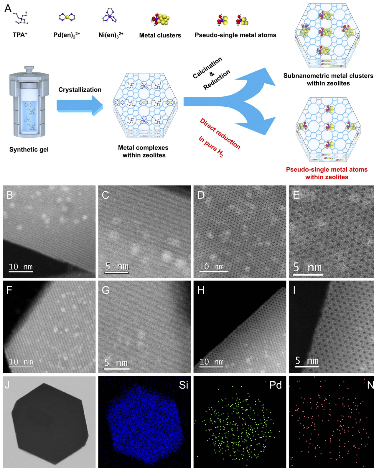
Fig. 1 (A) Schematic illustration of the preparation of zeolite-encaged Pd-based catalysts. \text{C}_\text{e} -corrected STEM images of (B and C) \text{Pd@S-1-C} ; (D and E) 0.8\text{Pd}0.2\text{Ni}(\text{OH})_2\text{@S-1-C} ; (F and G) \text{Pd@S-1-H} ; (H and I) 0.8\text{Pd}0.2\text{Ni}(\text{OH})_2\text{@S-1-H} . (J) TEM image of 0.8\text{Pd}0.2\text{Ni}(\text{OH})_2\text{@S-1-H} catalyst and corresponding EDX mapping images for Si, Pd, and Ni elements. Scale bar: 250 nm.
