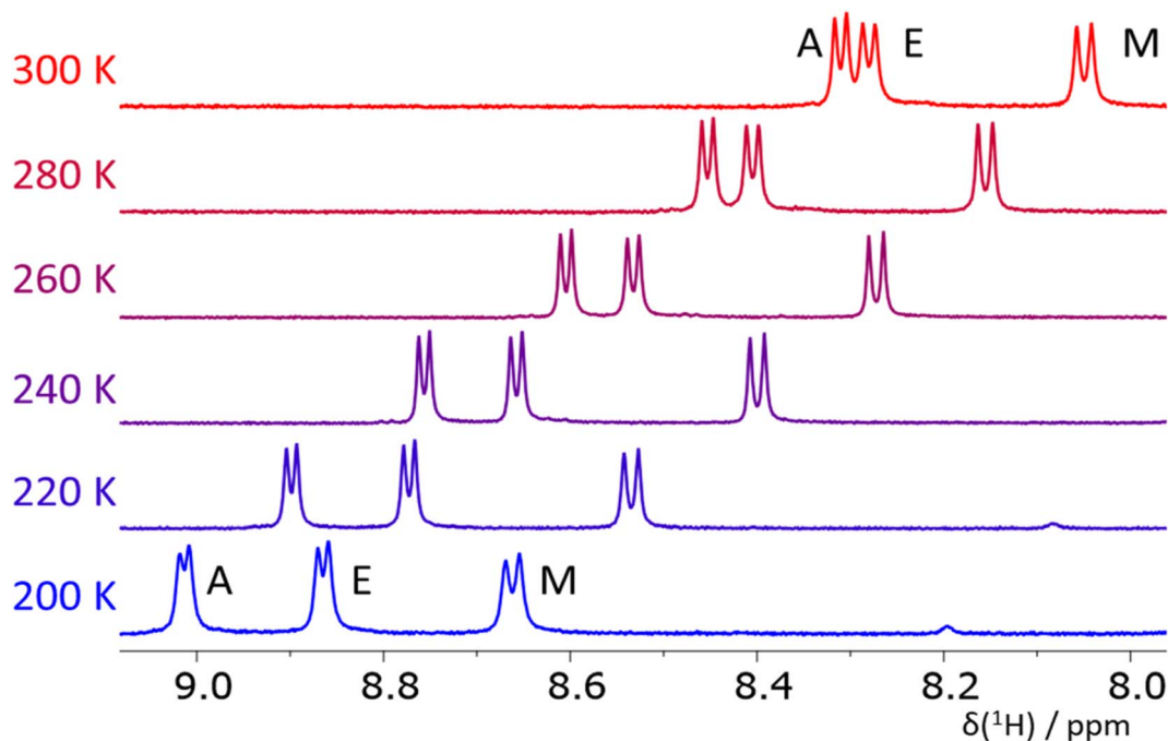
Fig. 6 The NH region of ^1\text{H} NMR spectra of the tripeptide EAM in methanol at T = 200 – 300\text{ K} . The temperature-induced changes in chemical shifts of the signals are caused by an intermolecular exchange of the NH and solvent protons.
