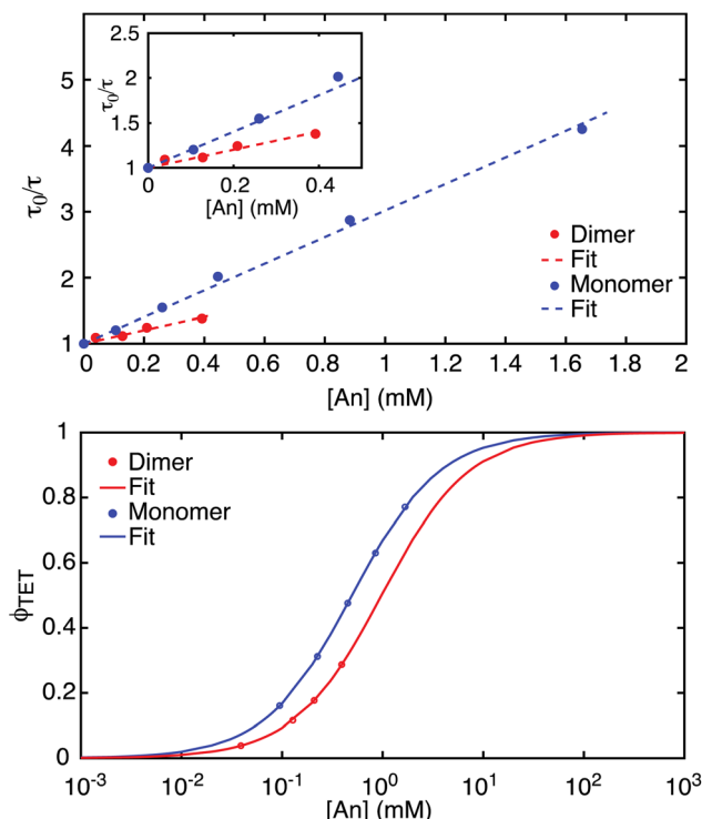
Fig. 3 (Top) Stern–Volmer plot for TIPS-BTX and TIPS-Tc in room-temperature toluene. Slopes reflecting K_{SV} along with sensitizer lifetime leads to values of k_{\text{TET}} = 3.0 \times 10^8 \text{ M}^{-1} \text{ s}^{-1} for TIPS-BTX and k_{\text{TET}} = 5.9 \times 10^8 \text{ M}^{-1} \text{ s}^{-1} for TIPS-Tc. The inset focuses on the lower annihilator concentration regime. (Bottom) Concentration dependent triplet energy transfer (TET) yields from Eq. 1c for TIPS-BTX and TIPS-Tc in room-temperature toluene.
