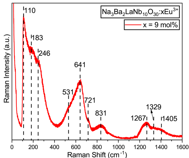
Fig. 10 Raman spectrum of the \text{Na}_3\text{Ba}_2\text{LaNb}_{10}\text{O}_{30}:\text{xEu}^{3+} ( x = 9 mol%) phosphor at room temperature.
