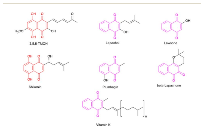
Fig. 1 Representative naphthoquinone-based important compounds.
