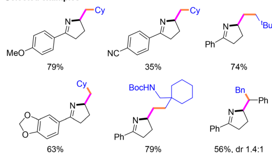
Scheme 15 Csp 3 –Csp 3 decarboxylated cross-coupling reaction via E T .
