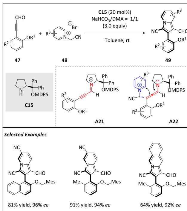
Scheme 16 Atroposelective intermolecular [8 + 2] cycloadditions via iminium-ion catalysis.
