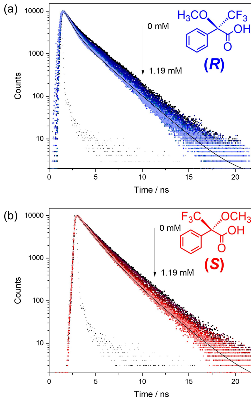
Fig. 4 Fluorescence decay curves for the BINOL fluorophore in acetonitrile alone (10 mM) and in the presence of an increasing concentration of (a) (R)-Mosher's Acid or (b) (S)-Mosher's Acid. The fluorescence was recorded using \lambda_{\text{ex}} = 300 nm and \lambda_{\text{em}} = 416 nm. The solid black line is the fit and the black data points the instrument response function (IRF).
