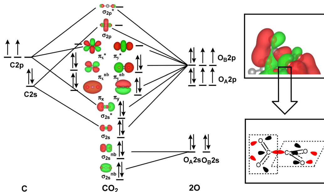
Fig. 4 The frontier molecular orbitals of free carbon dioxide molecules and the HOMO of the \ast\text{OCCO}\ast\text{O}\ast dimer, highlighting that the effective overlapping of two distorted \pi^\ast antibonding orbitals of two bent \text{CO}_2 molecules results in the formation of the C–C bond in the \text{CO}_2 dimer.
