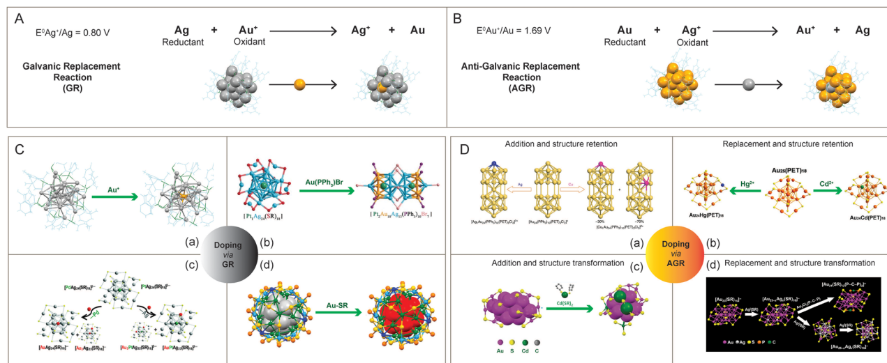
Fig. 7 Schematic representation of (A) galvanic replacement and (B) anti-galvanic replacement reaction from the context of doping in Ag 25 (SR) 18 and Au 25 (SR) 18 , respectively. Examples showing the preparation of alloy nanoclusters using (C) galvanic and (D) anti-galvanic reaction routes. Reproduced with permission from ref. C-a, 234 b, 236 c, 237 and d, 238 and D-a, 246 b, 248 c, 251 and d. 249 Copyright 2015 and 2017 American Chemical Society. Copyright 2016 and 2018 John Wiley and Sons. Copyright 2016 Royal Society of Chemistry. Copyright 2017, Springer Nature Group. Copyright 2019 National Academy of Sciences.
