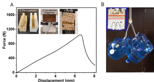
Fig. 7 (A) Tensile result of the bench-scale prefabricated joints connected by our cured elastomer, along with the protocol of setting up the bench-scale prefabricated joint. (B) Illustration of the ultra-high adhesion performance of our ductile adhesive elastomer using the bench-scale prefabricated joints.
