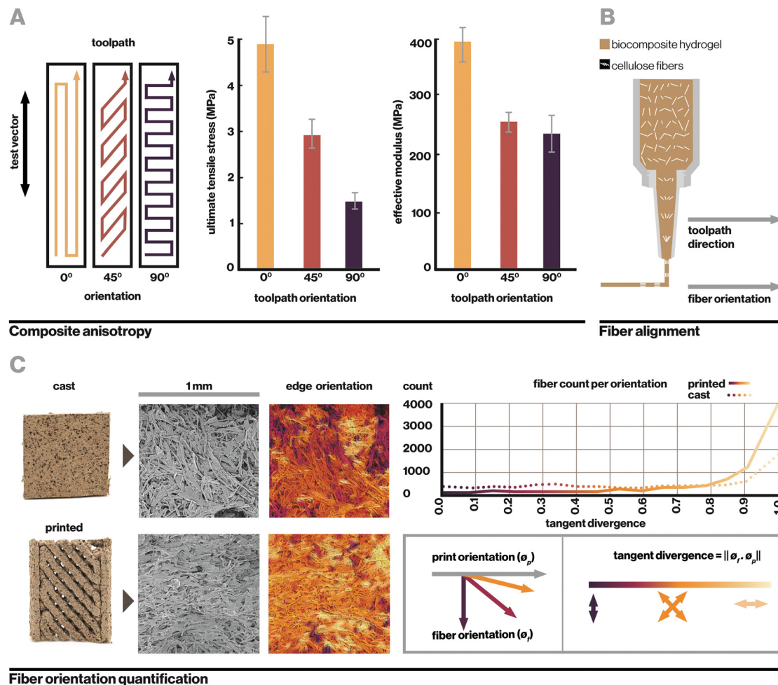
Fig. 3 Additive manufacturing creates hierarchical anisotropy that impacts mechanical properties. (A) Toolpath orientation creates macroscale printed filament alignment. This, along with microscale cellulose alignment, creates anisotropy in printed composites, with greatest ultimate tensile stress and Young's Modulus measured along the axis of print orientation. (B) Shear stress in the extrusion process forces microscale alignment of cellulose fibers in the same orientation as the toolpath direction. (C) Fiber alignment was quantified by visualizing cellulose fibers with SEM and measuring their dominant angle of alignment via the average tangent. The divergence of this tangent from the print orientation provides a quantification of whether fibers align with the toolpath. The printed sample shows high fiber alignment with the print orientation. The cast sample, which is expected to have randomly oriented fibers, shows a lower level of alignment that may result from manually spreading the material during the casting process.
