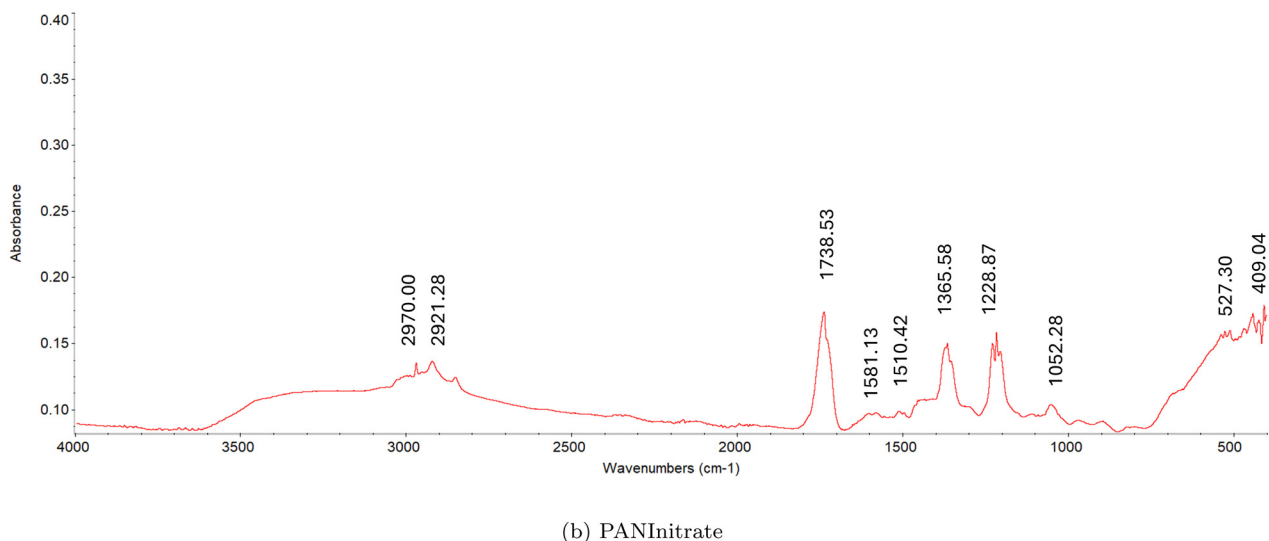
Fig. 20 FT-IR spectra of PANI synthesized using (a) ammonium persulfate (PANIAPS) and (b) ferrous nitrate (PANInitrate) as oxidizing agents.
