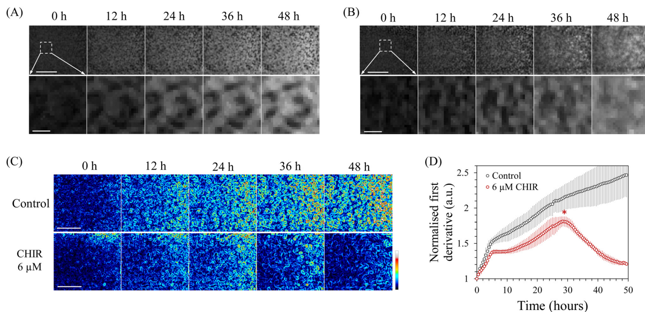
Fig. 3 Quantification of morphological change of colonies during mesoderm induction: (A and B) cropped INSPCTOR image of a control sample (A) and 6 \mu\text{M} CHIR treated sample (B). The top images show almost all of a region within a chamber, and the bottom images zoom in on the dot square area in the top image. (C) Visualisation of intensity gradient by normalised first derivative images of (A top) and (B top). Pixel intensity is visualised as colour. (D) Quantification of change in mean intensity of the normalised first derivative images. The asterisk represents the timing of morphological change corresponding to the initiation of EMT. Error bars represent standard deviation ( n = 4 ). Scale bars: 3 mm in A top, B top, and C, 500 \mu\text{m} in A bottom and B bottom.
