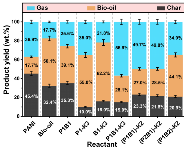
Fig. 1 The yields of gas, biochar/activated carbon and bio-oil from the pyrolysis or activation of polyaniline, bio-oil or their mixture of different mass ratios at 800 °C. P1B1: PANI and bio-oil mixed at a mass ratio of 1:1; P1-K3: PANI and K_2C_2O_4 mixed at a mass ratio of 1:3; B1-K3: bio-oil and K_2C_2O_4 mixed at a mass ratio of 1:3; P1B1-K3: PANI, bio-oil and K_2C_2O_4 mixed at a mass ratio of 1:1:3; (P1B1)-K2: PANI and bio-oil pre-polymerized at a ratio of 1:1 and then mixed with K_2C_2O_4 at a ratio of 1:2; (P2B1)-K2: PANI and bio-oil pre-polymerized at a ratio of 2:1 and then mixed with K_2C_2O_4 at a ratio of 1:2; (P1B2)-K2: polyaniline and bio-oil pre-polymerized at a ratio of 1:2 and then mixed with K_2C_2O_4 at a ratio of 1:2.
