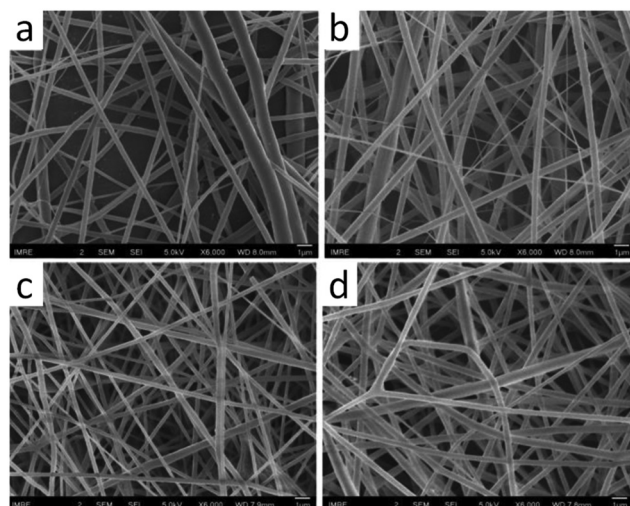
Fig. 23 SEM images of electrospun (a) PCL, (b) PCL/LP1, (c) PLLA, and (d) PLLA/LP1 nanofibers. Scale bars = 1 μm. Reproduced from ref. 143 with permission from American Chemical Society, copyright 2017.
