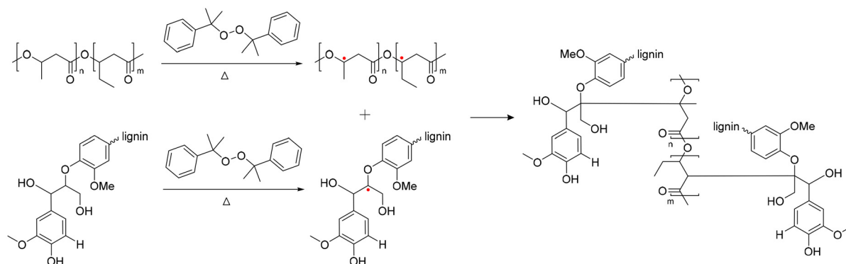
Scheme 18 Synthesis of lignin-graft-PHBV. Terminal β-O-4 softwood lignin unit is used for simplicity.
