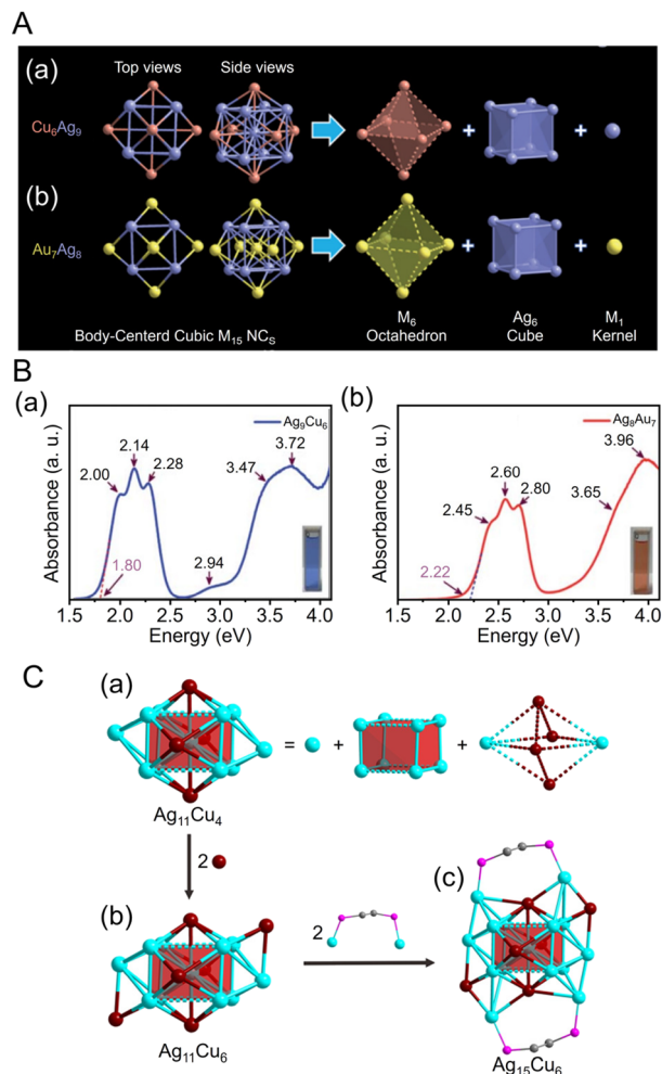
Fig. 13 (A) Anatomy of (a) [Ag_9Cu_6(C\equiv C'Bu)_{12}]^+ and (b) [Ag_8Au_7(C\equiv C'Bu)_{12}]^+ . Color legend: Au, yellow; Ag, purple; Cu, orange. (B) Experimental absorbance spectra plotted in the energy axis of (a) [Ag_9Cu_6(C\equiv C'Bu)_{12}]^+ and (b) [Ag_8Au_7(C\equiv C'Bu)_{12}]^+ . (C) Structure analysis of the [Ag_{15}Cu_6(C\equiv C'Bu)_{12}]^+ . (a) Structure anatomy of the Ag_{11}Cu_4 metal core. (b) Capping of two opposite Ag_3 faces of the Ag_{11}Cu_4 core forms the structure of Ag_{11}Cu_6 . (c) Stabilization of the Ag_{11}Cu_6 metal framework by two Ag_2DPPE motifs forms the structure of [Ag_{15}Cu_6(C\equiv C'Bu)_{12}]^+ . Color legend: turquoise, Ag; dark red, Cu; pink, P; gray, C. (A) and (B) are reproduced with permission from ref. 244. Copyright 2021 Royal Society of Chemistry. (C) is reproduced with permission from ref. 263. Copyright 2022 American Chemical Society.
