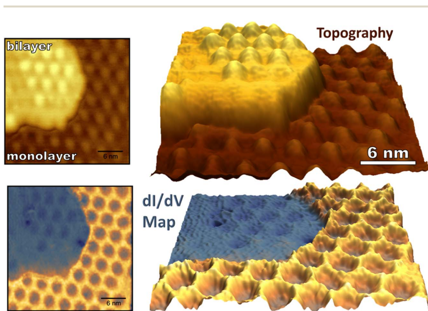
Fig. 5 Topography (top) and conductance mapping (bottom) of pristine monolayer and bilayer graphene on Ru(0001) is shown (−1.5 V, −250 pA). The bias was modulated with an amplitude of 200 mV to generate the dI/dV map. Note that atop regions of the single-layer graphene moiré pattern and the entirety of the bilayer graphene show lower conductance than the HCP and FCC regions of the G/Ru(0001) moiré pattern.
